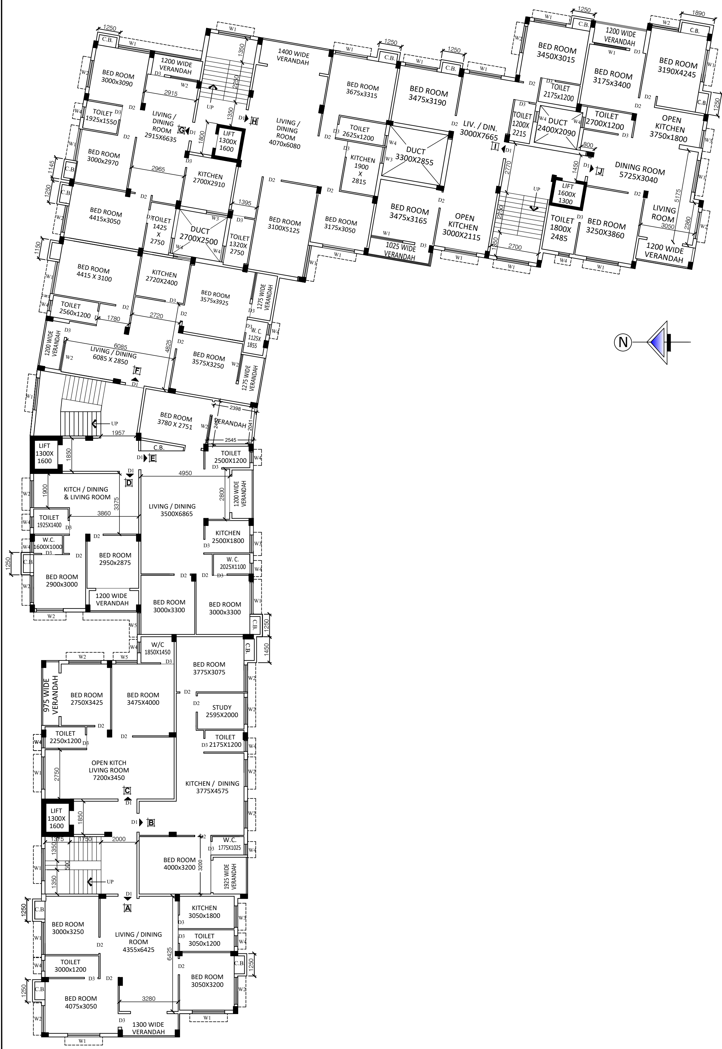
4TH FLOOR PLAN SCALE - 1 : 100.
